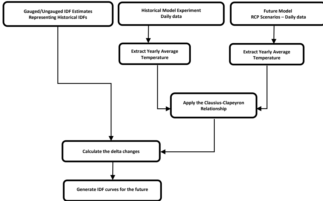
Figure 7: The Clausius-Clapeyron relationship with temperature scaling for generating future IDF curves under climate change for gauged/ungauged IDF curves
